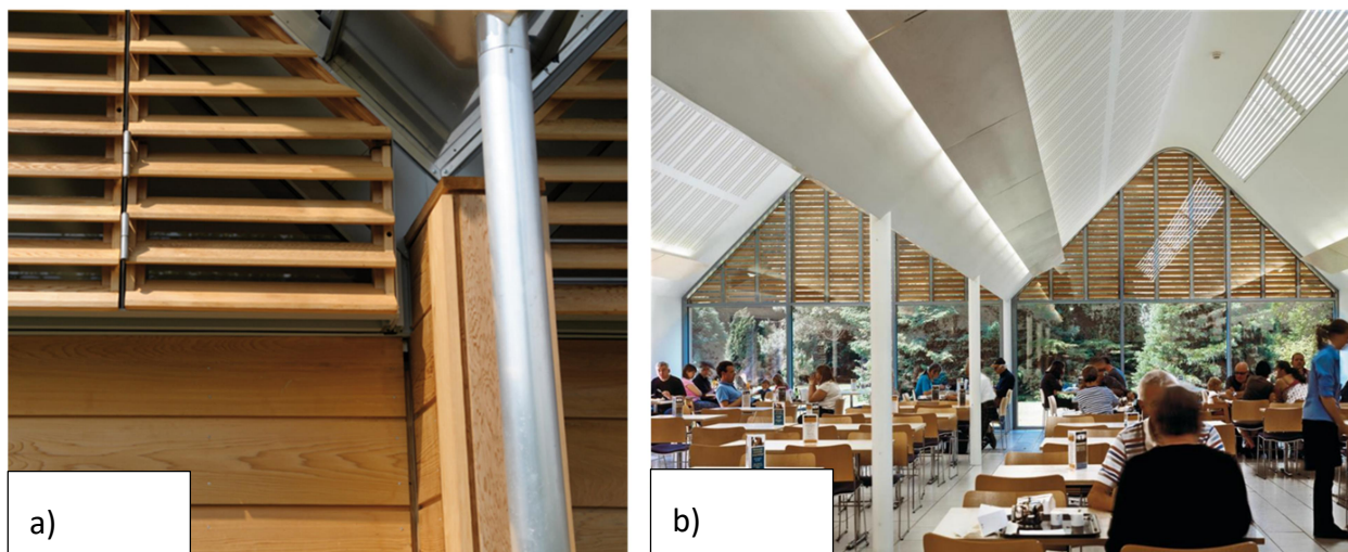
Fig. 3.18. Anglesey Abbey Visitor Centre: a) Close up of hinged louvre detail on elevation (TRADA, 2019); b) View inside restaurant (Detail, 2009)
