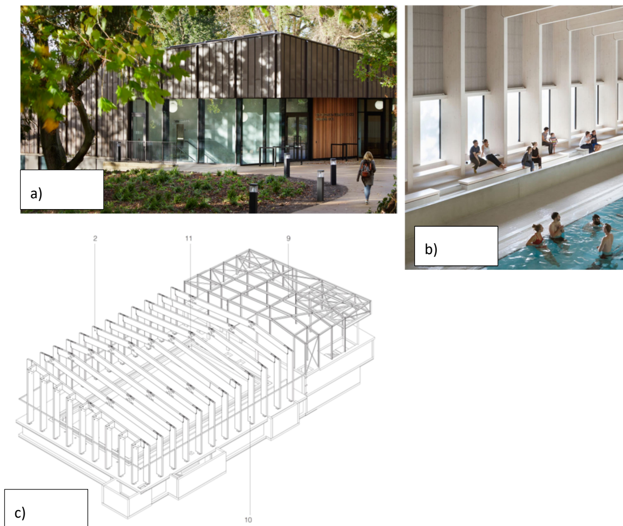
Fig. 3.16. City Of London Freeman's School Swimming Pool: a) Building is clad with dark copper-coloured zinc panels. (Hawkins Brown, 2018); b) The white-stained glulam frames and CLT panels create a light and spacious pool; c) Isometric view of pool structure (Hawkins Brown, 2018)
