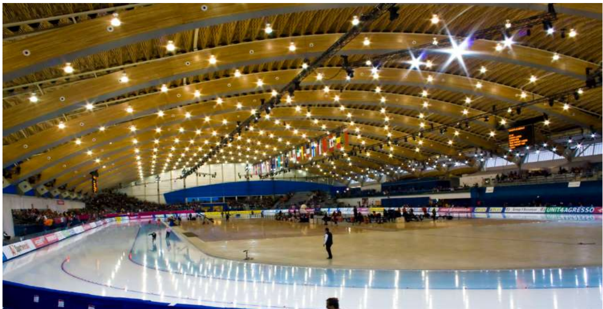
Fig.3.26. Richmond speed skating rink
